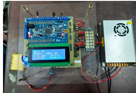
Figure 13. System implementation for charging RC car battery
