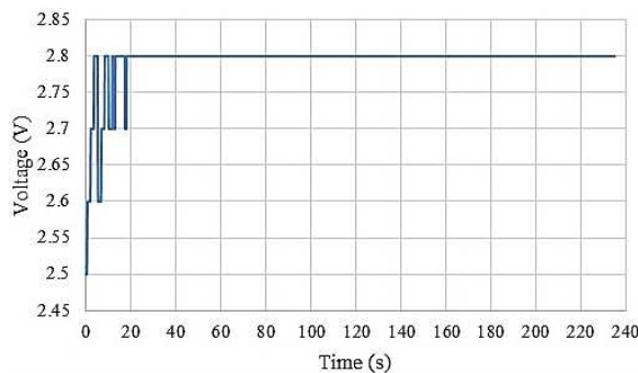
Figure 8. Graph of charging mosquito racket battery
