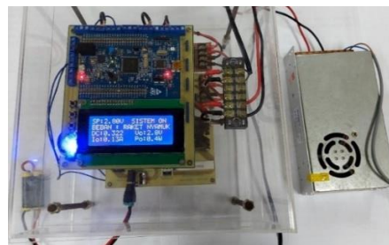
Figure 7. System implementation for charging mosquito racket battery
