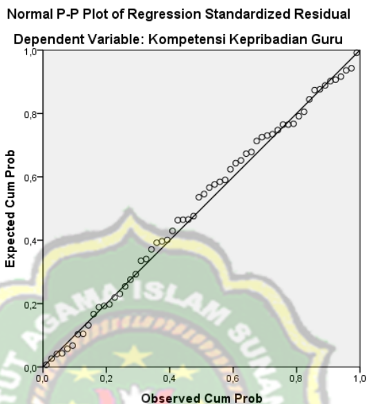
Gambar 4.3 Grafik Probability Plot Uji Normalitas Data
