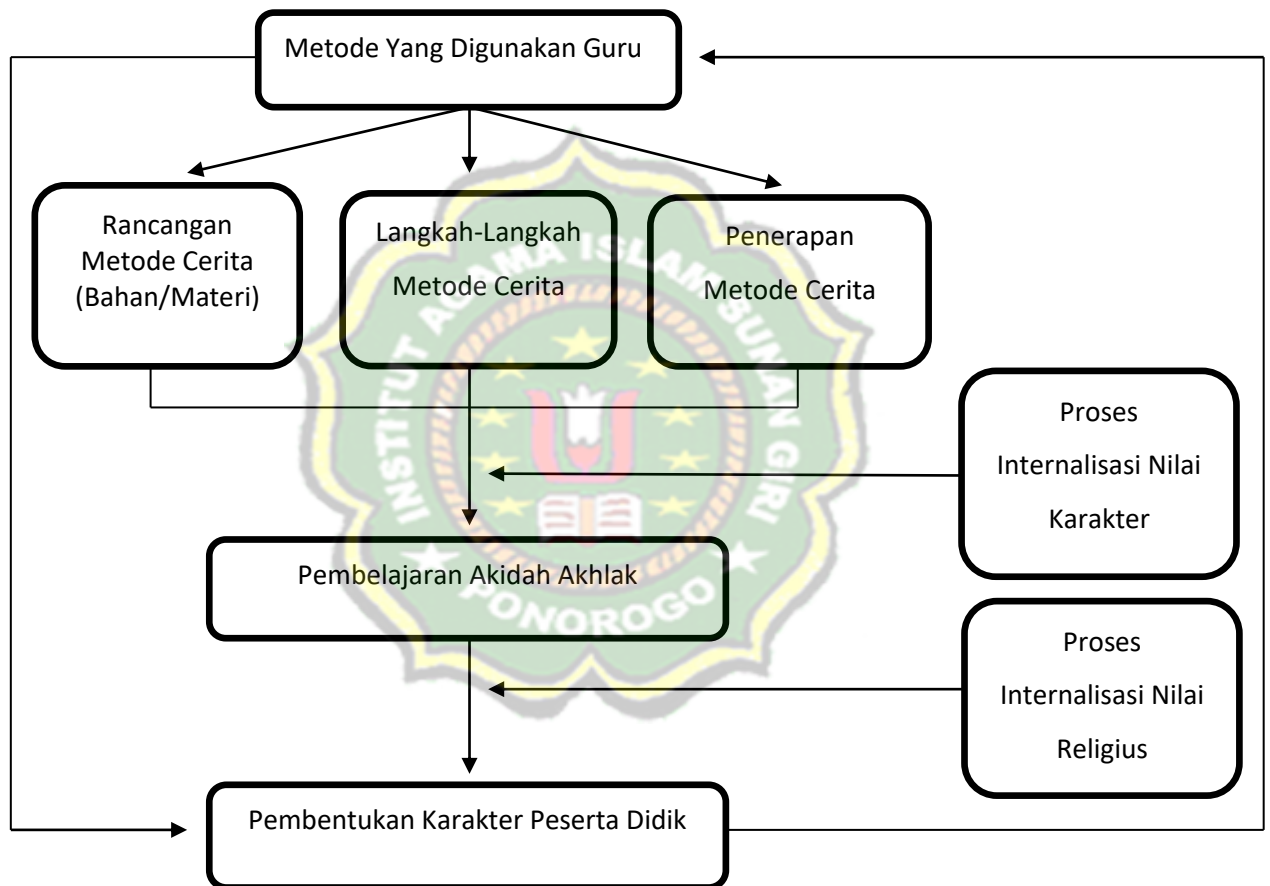
Gambar 2.1 : Paradigma Penelitian
